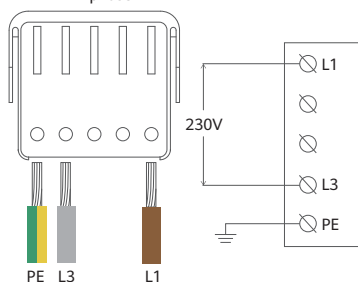
IT 1-phase
